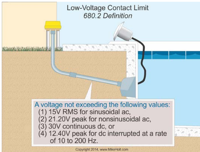
Figure 680-4
