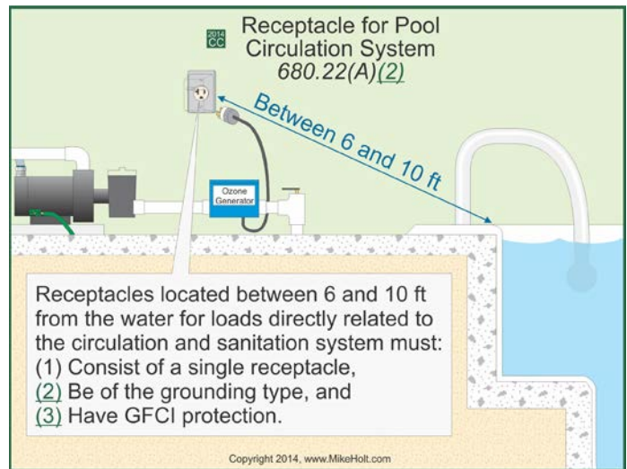
Figure 680-23
