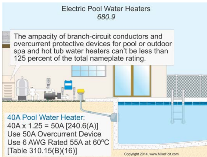
Figure 680-13
