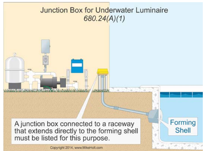
Figure 680-34
