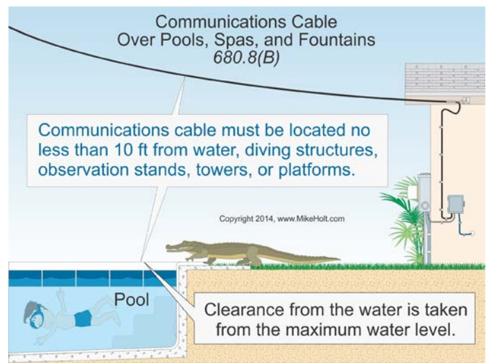
Figure 680-12
