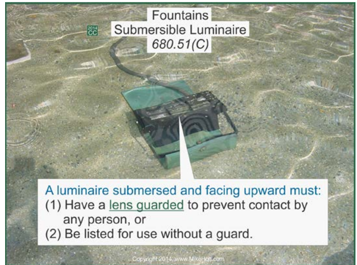
Figure 680–61
