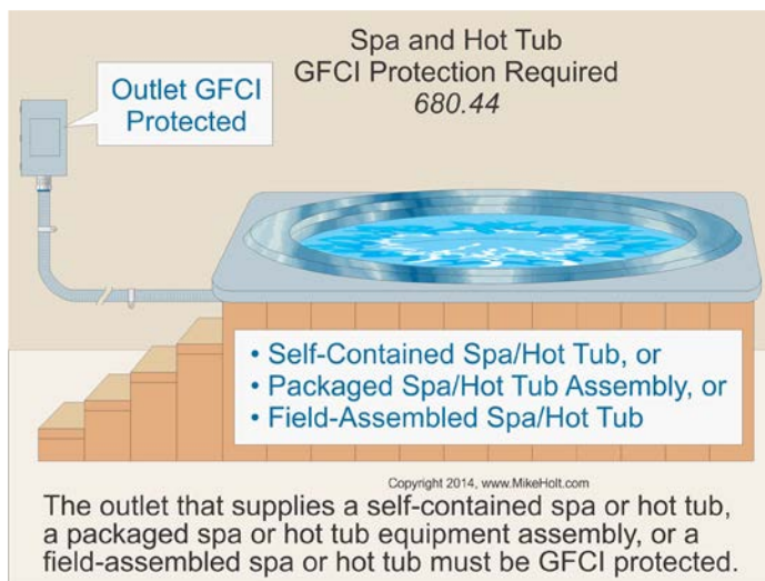
Figure 680–58
