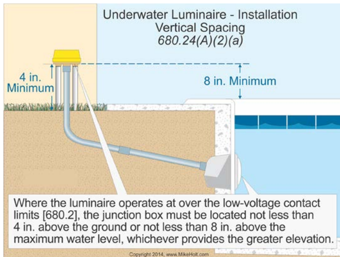
Figure 680–35
