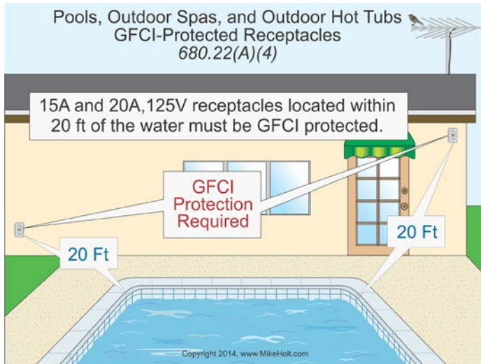
Figure 680-25
