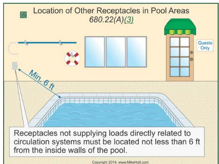
Figure 680-24
