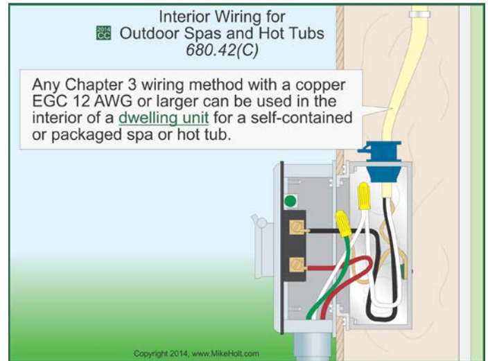
Figure 680-54
