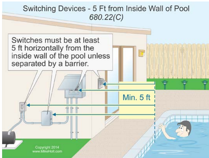
Figure 680–28
