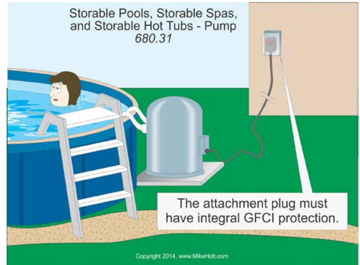
Figure 680–49
