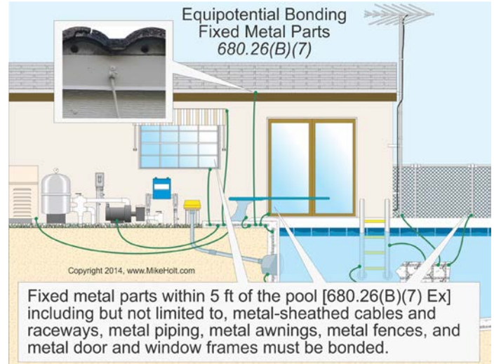
Figure 680–46
