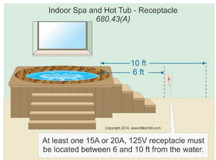
Figure 680-55
